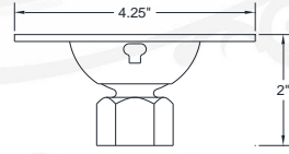
SLC 1/2" SLOPE CEILING CANOPY 1/2" SLC 3/4" SLOPE CEILING CANOPY 3/4" *(Slopes To 20 Degrees)
