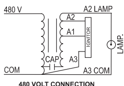
Wiring Diagram 32
