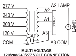
Wiring Diagram 29
