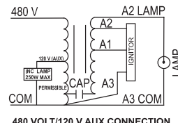
Wiring Diagram 33
