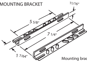
Mounting bracket for Core & Coil Ballasts (2 brackets with thru bolts)
