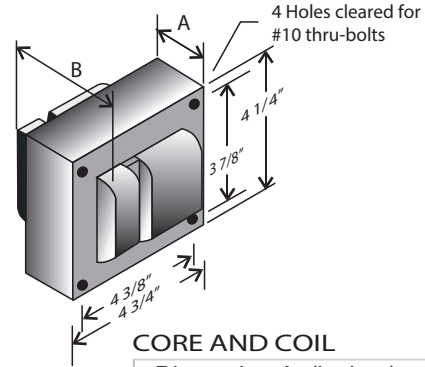
4 1/4" x 4 3/4" CORE
