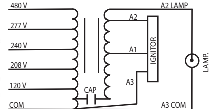
SUPER 5 120/208/240/277/480 VOLT CONNECTION
