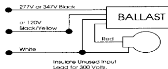
Wiring Diagram 34
