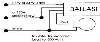
Wiring Diagram 34
